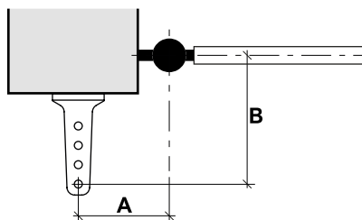
Abbild. D LEADER 4: D= max 175 mm
