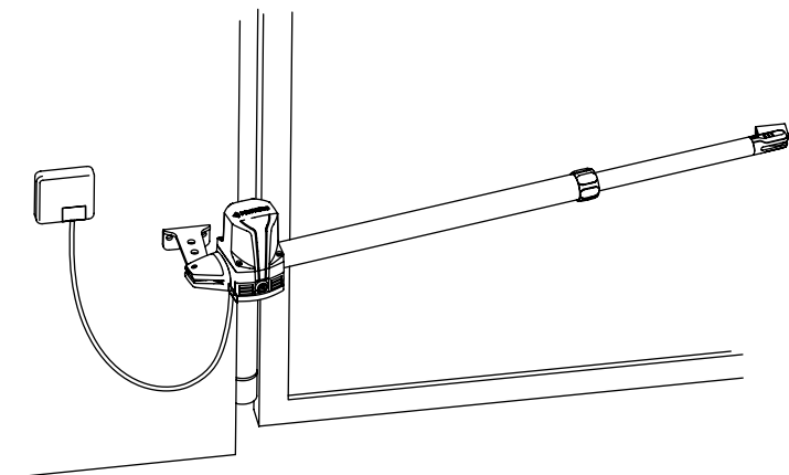
Abbild. D LEADER 4: D= max 175 mm
