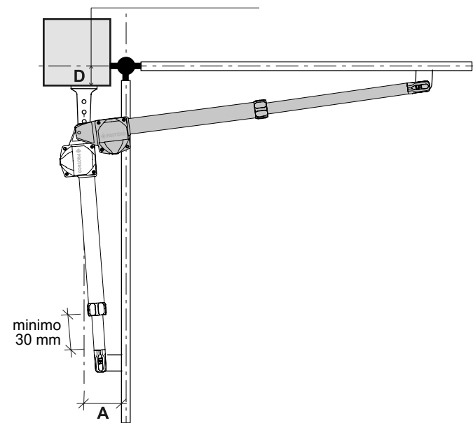
Abbild. D LEADER 4: D= max 175 mm
